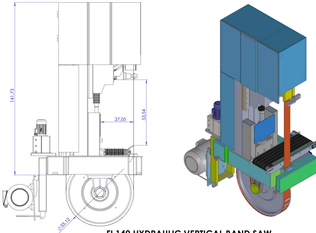
FI.140 HYDRAULIC VERTICAL BAND SAW
